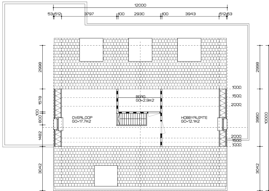
ZOLDER
